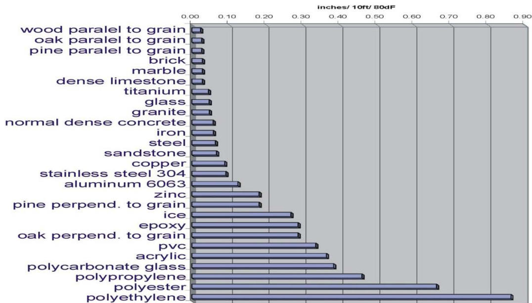
Figure 4. Thermal movement of a 10ft long piece of a material subjected to an 80°F temperature differential
